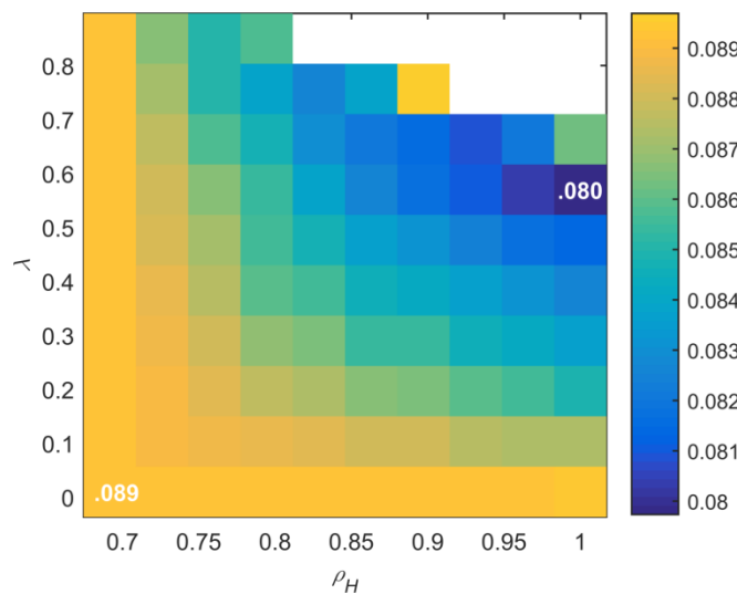
Figure A2. The left image illustrates the set of feasible policy vectors, \Omega_\lambda = (\rho_M, \rho_H, \lambda) , considered by the regulator. The right image illustrates each policy's corresponding interception rate cutoff z_\lambda . In both images, white cells represent policies that exceed the budget constraint. The left-most column represents the uniform policy.
